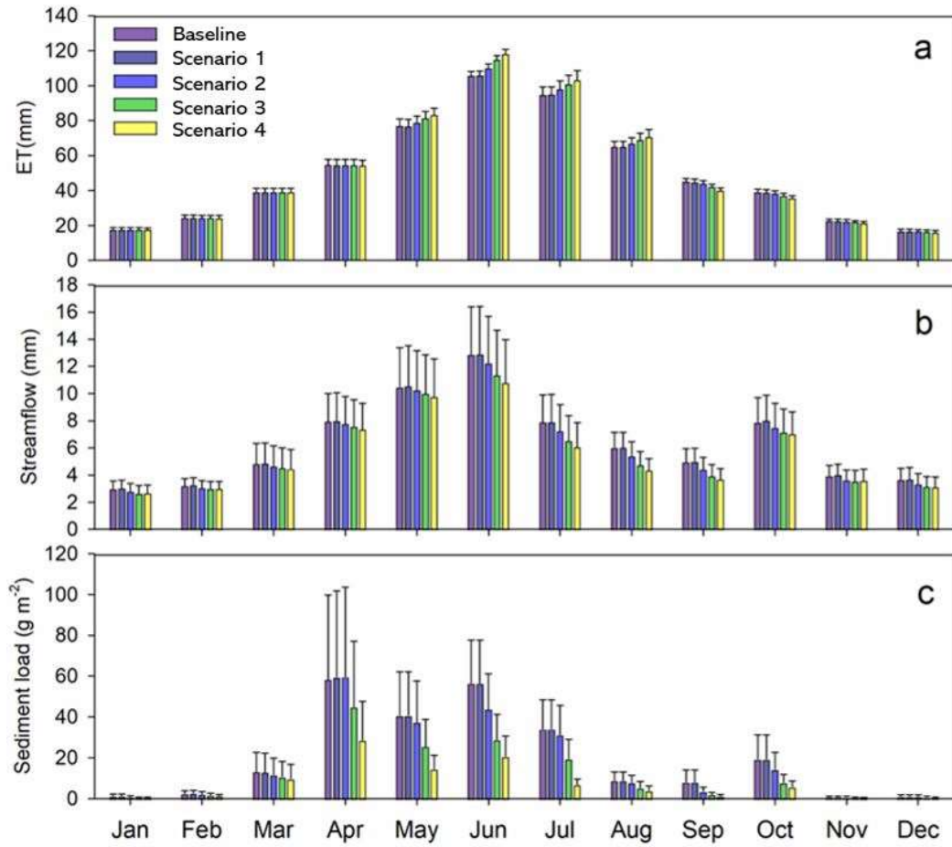
Figure S1. Average monthly (a) evapotranspiration, (b) streamflow, and (c) sediment yield during the model simulation period (2002–2018) for the baseline and four land use change scenarios in the Lower Cimarron River Basin, north-central OK, USA.
