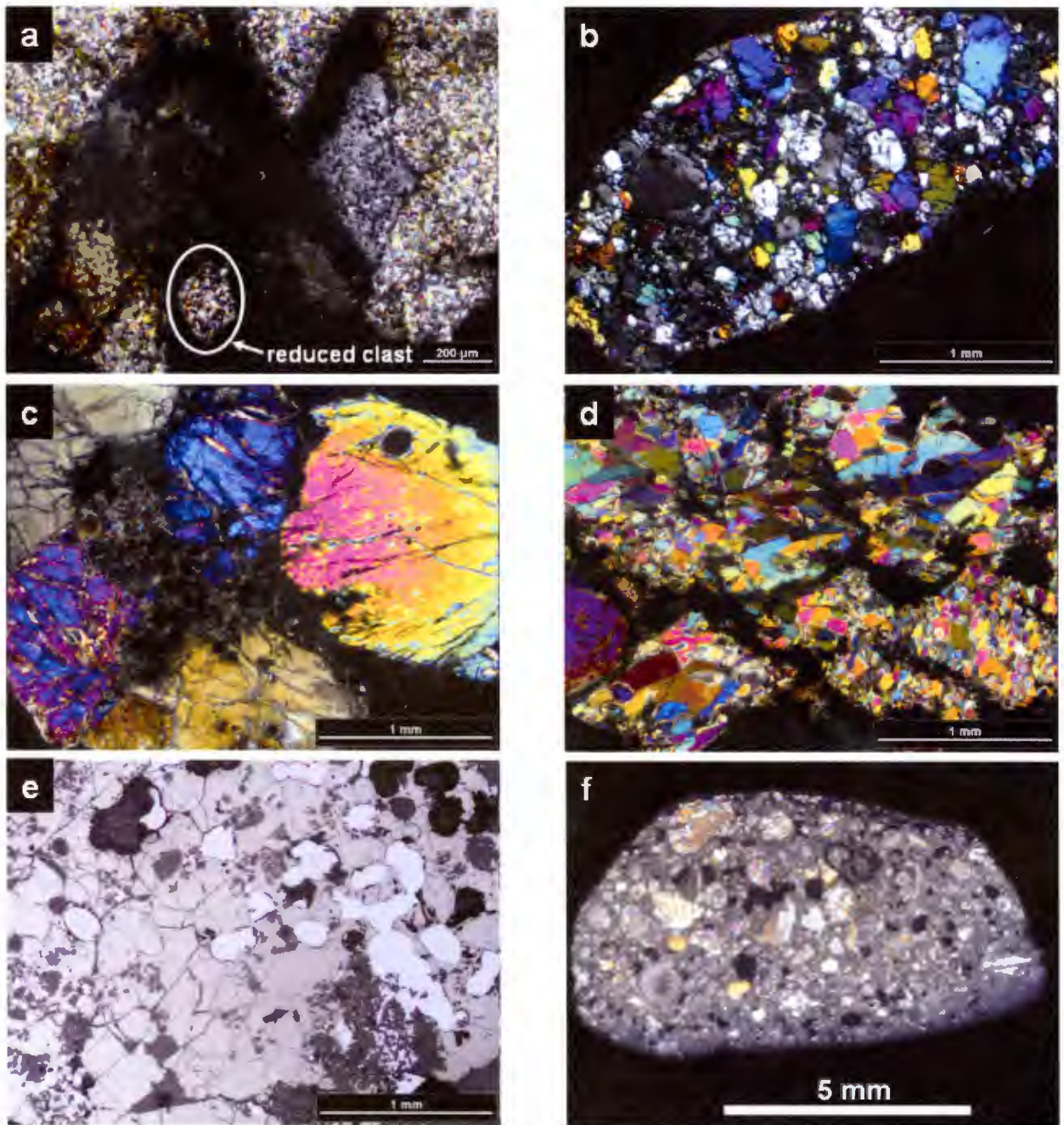
Figure 1: Photomicrographs in transmitted (crossed polarizers; (a)-(d), (f) and reflected (e) light: (a) Fragment MS-152 is a fine-grained, ureilitic object containing a reduced clast; Figs. (b)-(d) show some coarse-grained ureilites with different textures: (b) MS-153;
