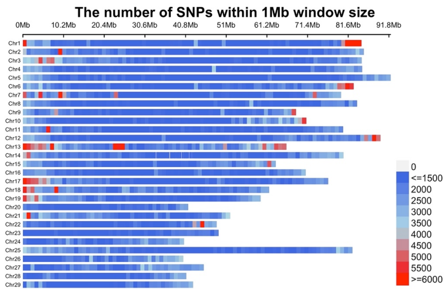
Supplemental Figure 1: SNP density for both Sashin (A) and Little Sheep Creek (B). Value is calculated from the number of SNPs over 1,000,000 base pair windows. Areas of low SNP density (Blue) indicate regions with either low sequencing coverage or substantial sequence overlap between migratory and resident O. mykiss , whereas red areas indicate regions of the genome with considerable differences between phenotypes.
