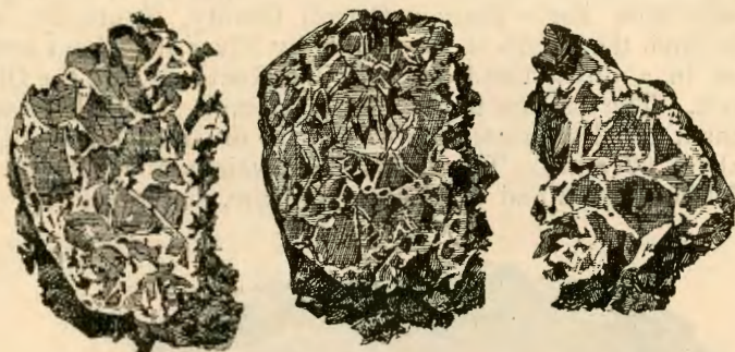
Sections of the Carroll County Meteorite. Natural size.
