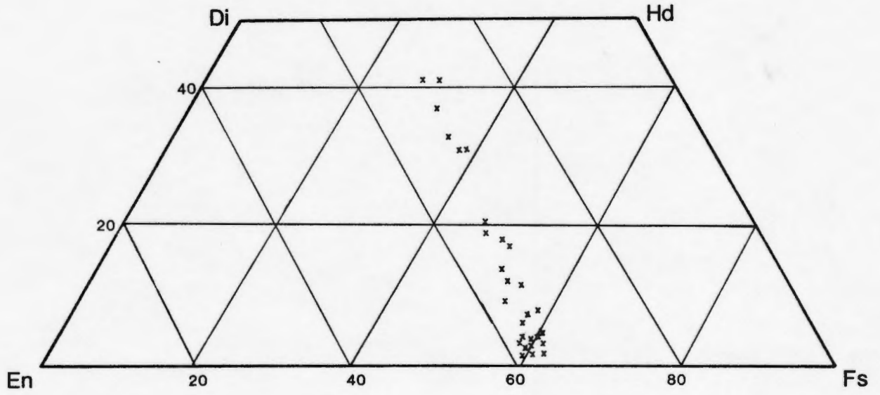
Fig. 5: Pyroxene compositions for the Kirbyville taken from microprobe data.
