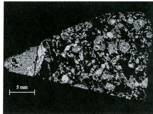
Figure 1. X-ray map for Mg K \alpha . 1024 \times 768 pixels. Dark gray – opx; light gray – olivine; black – very largely metal.
