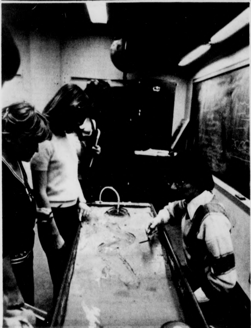
GOING WITH THE FLOW—Geology students observe the effects of running water on the environment in a stream experiment. The lab simulates stream and sediment movement. Observers can speed up natural processes with a simulator to study how various water velocities create geological phenomena.
