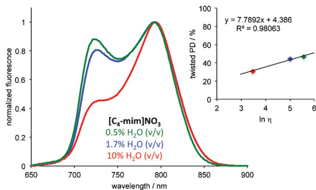
Fig. 5 Emission spectra of PD in [\text{C}_4\text{-mim}]\text{NO}_3 as a function of the water content. Inset: effect of [\text{C}_4\text{-mim}]\text{NO}_3 viscosity (red symbol – 10% of \text{H}_2\text{O} ; blue symbol – 1.7% of \text{H}_2\text{O} and green – 0.5% of \text{H}_2\text{O} ) as a function of PD conformation. Conditions: [\text{PD}] = 1 \mu\text{M} , \lambda_{\text{ex}} = 475 \text{ nm} , [\text{DMSO}] = 0.1\% \text{ (v/v)} .
